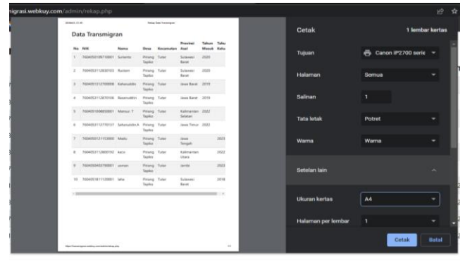
Gambar 4.5 Form login
