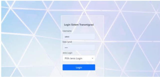
Gambar 4.2 Form login
