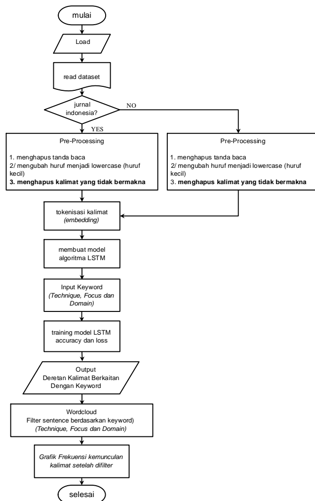
Gambar 1 Flowchart Model LSTM
